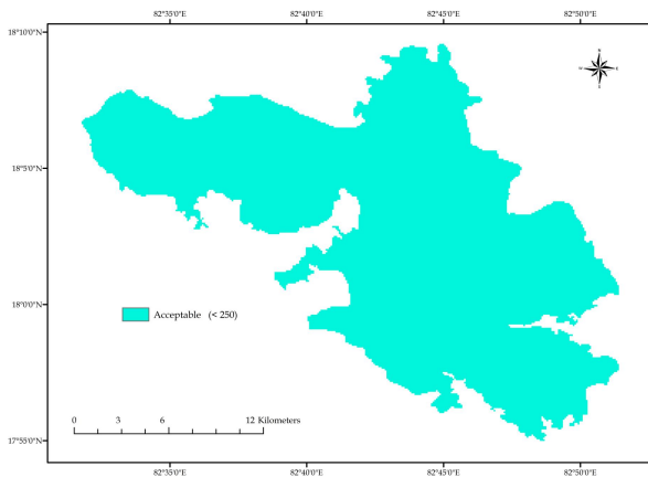
Figure 6. Spatial distribution of Chloride ( \text{Cl}_2^- )
