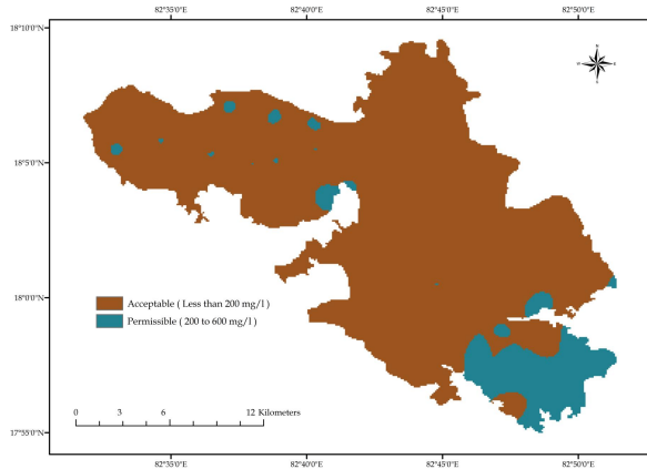
Figure 4. Spatial distribution of Total Hardness
