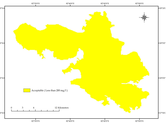
Figure 7. Spatial distribution of Sulphate ( \text{SO}_4^{2-} )
