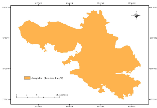
Figure 8. Spatial distributions of Fluoride (F - )
