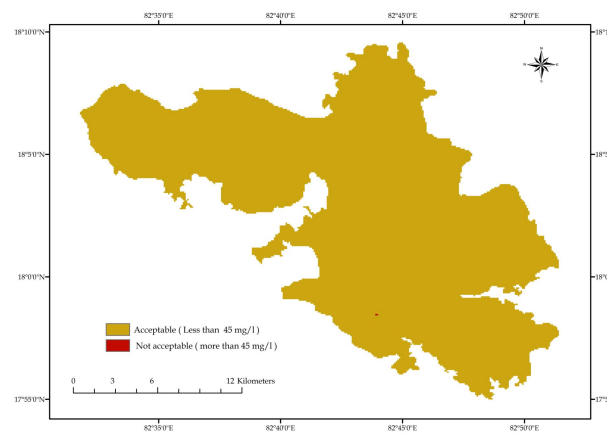
Figure 9. Spatial distribution of Nitrate (NO 3 - )
