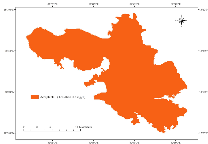
Figure 10. Spatial distribution of Iron (Fe)
