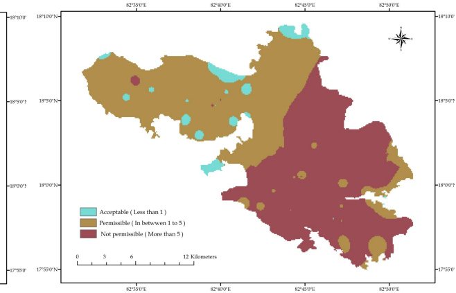
Figure 5. Spatial distribution of turbidity
