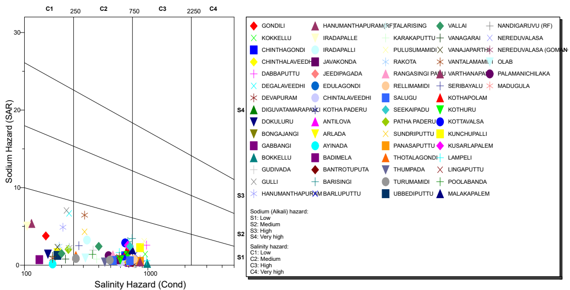
Figure 12. Sodium Hazard
