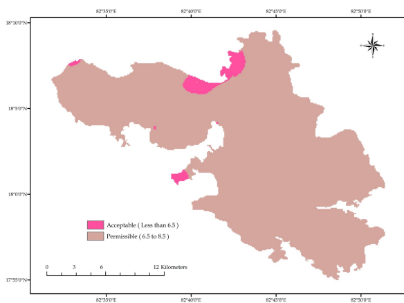
Figure 2. Spatial distribution of pH
