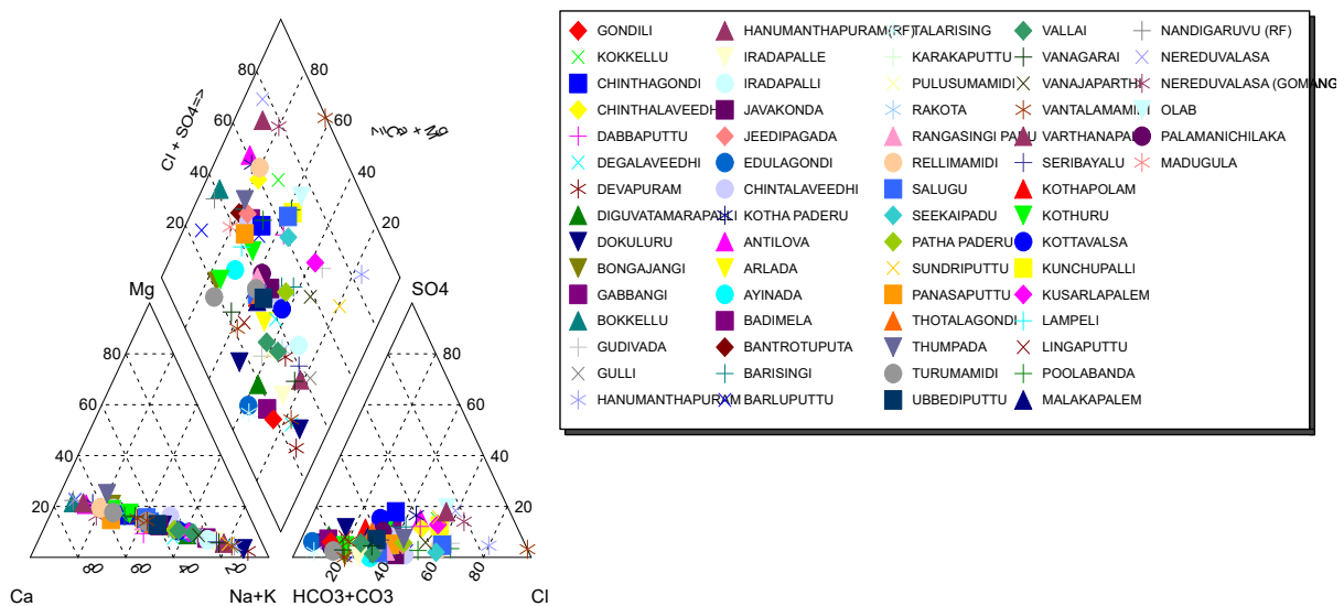
Figure 11. Hill-Piper diagram
