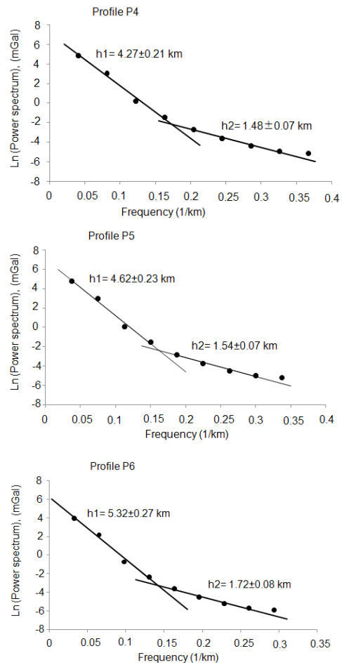
Figure 9. Power spectra of profiles P4, P5, and P6 of the Mayo Oulo-Lere sedimentary basin.
