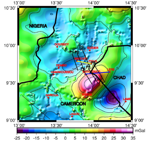
Figure 7. Fourth-order of residual Bouguer anomaly map of the region obtained after combining the terrestrial gravity data and the EGM2008 model. Black, yellow, and blue lines represent geological faults, and the Babouri-Figuil and Mayo Oulo-Lere sedimentary basins, respectively.
