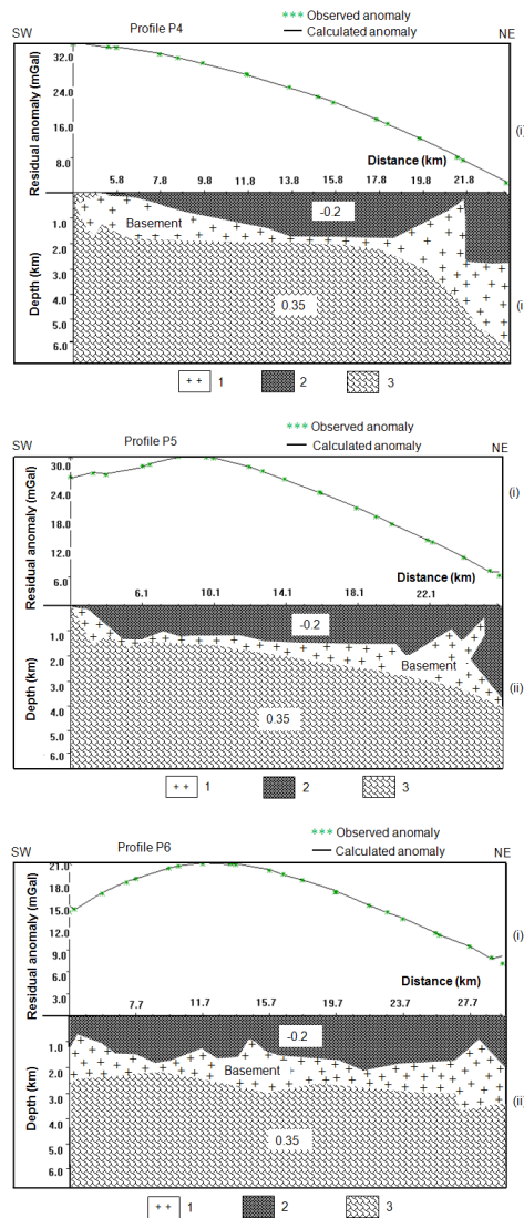
Figure 11. Crustal model of profiles P4, P5, and P6 of the Mayo Oulo-Lere sedimentary basin.
