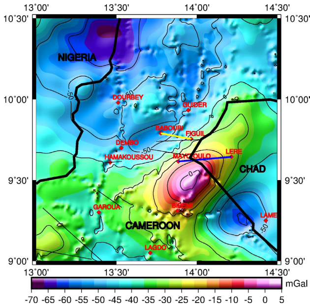
Figure 4. Bouguer anomaly map of the region obtained after combining terrestrial gravity data and the EGM2008 model. Black, yellow, and blue lines represent geological faults, and the Babouri-Figuil and Mayo Oulo-Lere sedimentary basins, respectively.
