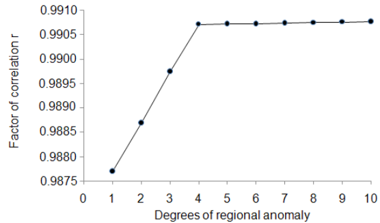
Figure 6. The factor of correlation according to the degrees of regional anomaly.
