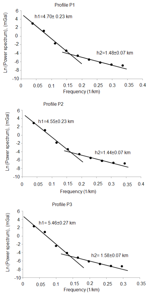
Figure 8. Power spectra of profiles P1, P2 and P3 of the Babouri-Figuil sedimentary basin.
