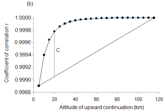
Figure 5. Optimum upward-continuation height by the method of Zeng et al. [16]. (a) Cross-correlation between two successive upward-continued heights as a function of the continuation height. (b) The deflection C of the cross-correlation curve.
