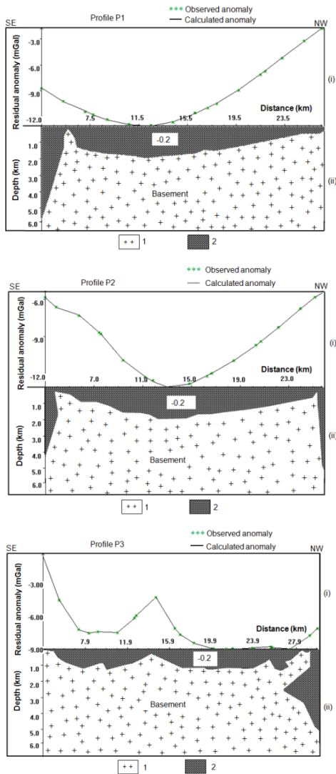
Figure 10. Crustal model of profiles P1, P2, and P3 of the Babouri-Figuil sedimentary basin.
