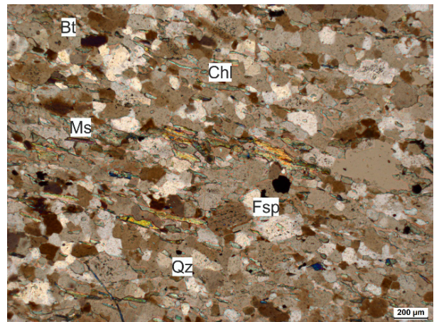
Figure 5. Phyllite (HR63) shows a mineral assemblage of biotite, muscovite, chlorite, feldspar and quartz (Abbreviations are after Whitney and Evans, 2010) [26] .
